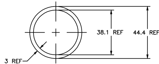
△ O'RING DETAIL
